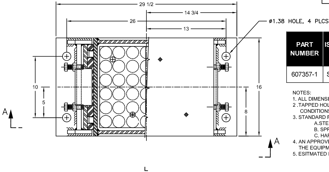
PLAN SECTION "B-B"
